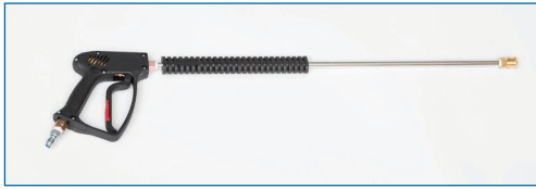
#353033 - Suttner Gun Assembly 28" Wand #353038 - Suttner Gun Assembly 36" Wand
