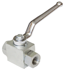
High Pressure Ball Valve #2517 - 1/4" FPT 7,000 PSI #4997 - 3/8" FPT 7,000 PSI #4998 - 1/2" FPT 7,000 PSI #410099 - Replacement Handle
